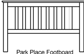
Park Place Footboard Available in Twin, Full & Queen sizes 5367T - 41" wd x 3" dp x 36" hi 5367F - 59" wd x 3" dp x 36" hi 5367Q - 65" wd x 3" dp x 36" hi
